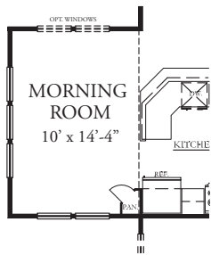
OPT. MORNING ROOM NOT AVAILABLE ON ALL HOMESITES
