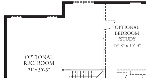
PARTIAL FOUNDATION PLAN W/ OPT. 4'-0" GREAT ROOM EXTENSION AND OPT. 4'-0" OWNER'S BEDROOM EXTENSION
