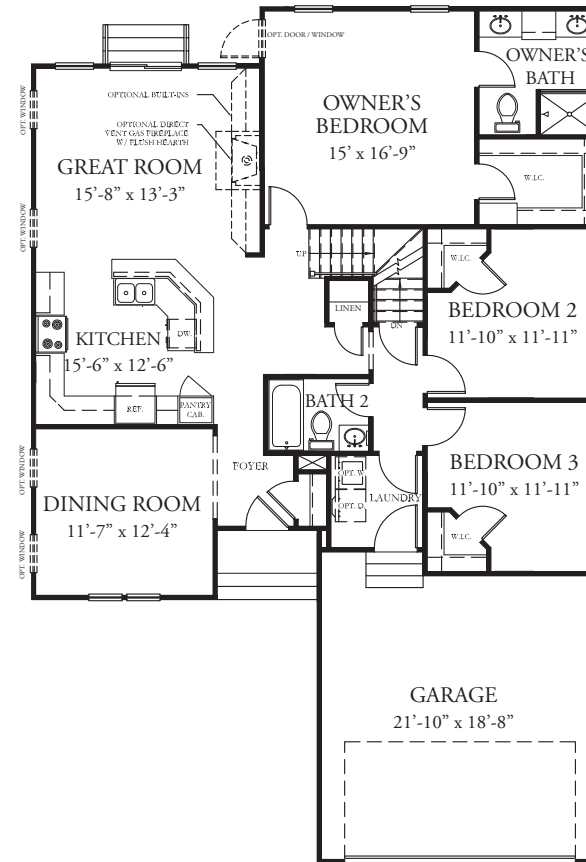
FIRST FLOOR PLAN SHOWN W/ LOWER LEVEL & SECOND LEVEL
