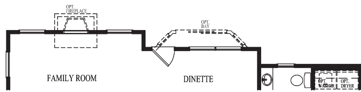
PARTIAL FIRST FLOOR PLAN W/ OPT. 4' EXTENDED FAMILY ROOM
