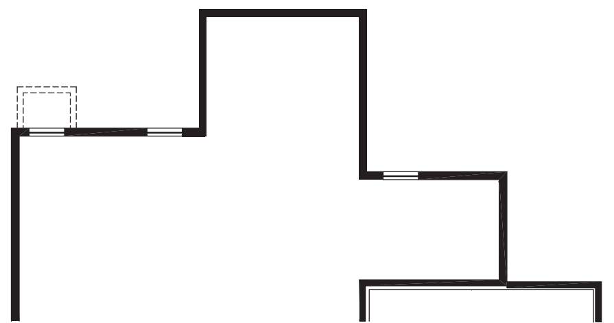
PART. OPT. LOWER LEVEL PLAN W/OPT. 4' EXTENDED FAMILY ROOM & OPT. MORNING ROOM
