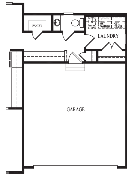
PARTIAL FIRST FLOOR PLAN W/ OPT. ENLARGED LAUNDRY ROOM
