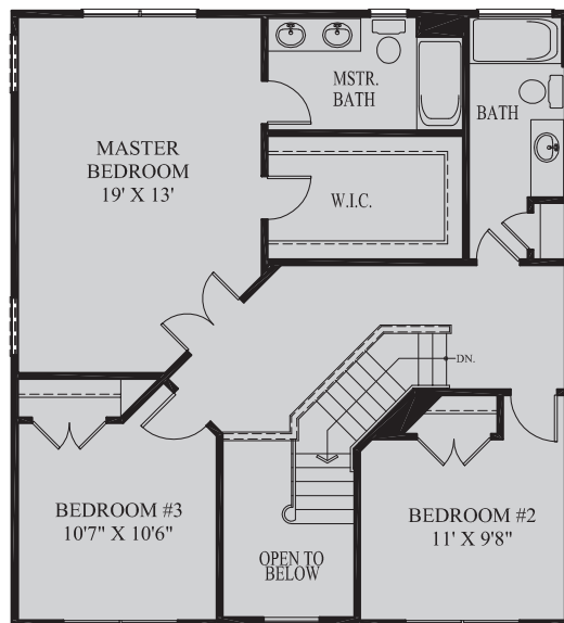
STD. SECOND FLOOR PLAN
