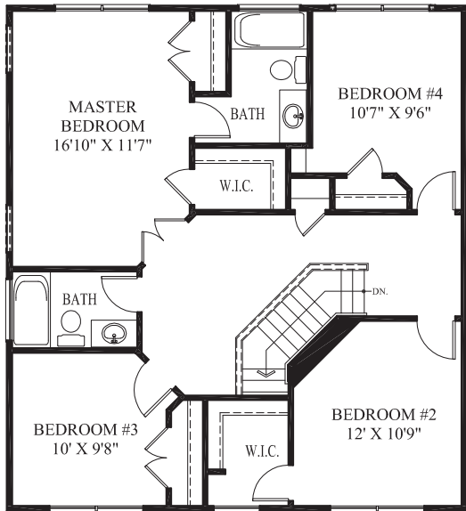
ALT. SECOND FLOOR PLAN W/ OPT. BEDROOM #4
