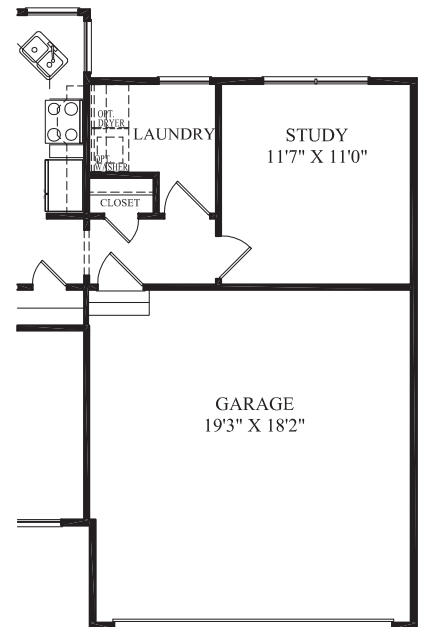
PARTIAL FIRST FLOOR PLAN W/ OPT. STUDY & FIRST FLOOR LAUNDRY
