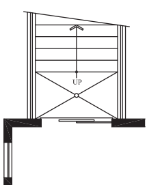
PARTIAL FND. PLAN W/ OPT. 7' WELLED EXIT
