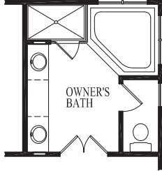
PARTIAL SECOND FLOOR PLAN W/ OPT. LUXURY MASTER BATH
