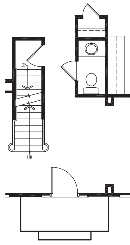
PART. FIRST FLOOR PLAN W/ OPT. BASEMENT
