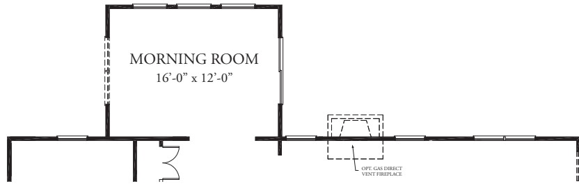
PARTIAL FIRST FLOOR PLAN W/ OPT. MORNING ROOM
