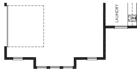
PARTIAL FIRST FLOOR W OPT. 3-CAR SIDE LOAD GARAGE AT ELEV. #3
