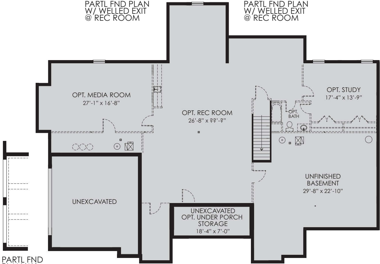
BASEMENT PLAN
